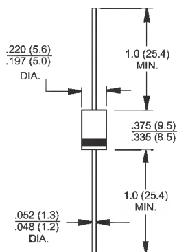
Dimensions in inches and (millimeters) Marking Diagram
